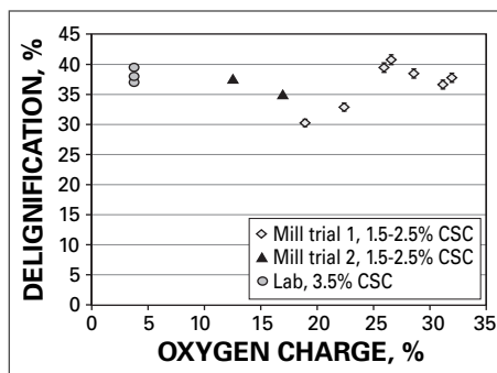
2. Softwood pulp before washers – delignification tests.
