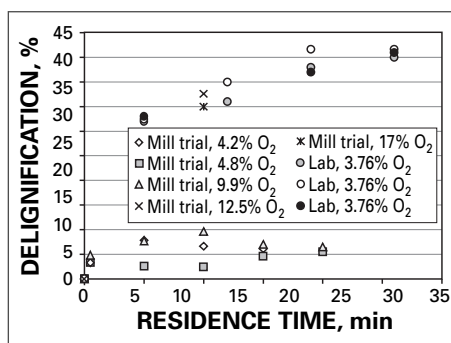
3: Delignification as a function of time.
